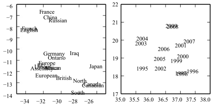
Figure 12.3: Two-dimensional visualizations of word embeddings obtained from a neural machine translation model (Bahdanau et al., 2015), zooming in on specific areas where semantically related words have embedding vectors that are close to each other. Countries appear on the left and numbers on the right. Keep in mind that these embeddings are 2-D for the purpose of visualization. In real applications, embeddings typically have higher dimensionality and can simultaneously capture many kinds of similarity between words.
