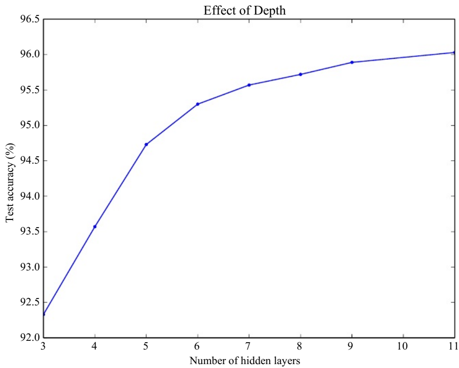
Figure 6.6: Empirical results showing that deeper networks generalize better when used to transcribe multi-digit numbers from photographs of addresses. Data from Goodfellow et al. (2014d) . The test set accuracy consistently increases with increasing depth. See Fig. 6.7 for a control experiment demonstrating that other increases to the model size do not yield the same effect.
