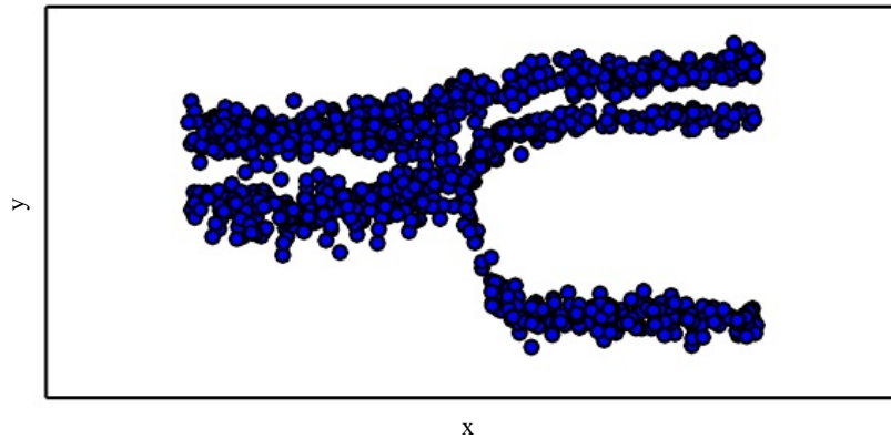
Figure 6.4: Samples drawn from a neural network with a mixture density output layer. The input x is sampled from a uniform distribution and the output y is sampled from p_{\text{model}}(y|x) . The neural network is able to learn nonlinear mappings from the input to the parameters of the output distribution. These parameters include the probabilities governing which of three mixture components will generate the output as well as the parameters for each mixture component. Each mixture component is Gaussian with predicted mean and variance. All of these aspects of the output distribution are able to vary with respect to the input x , and to do so in nonlinear ways.
