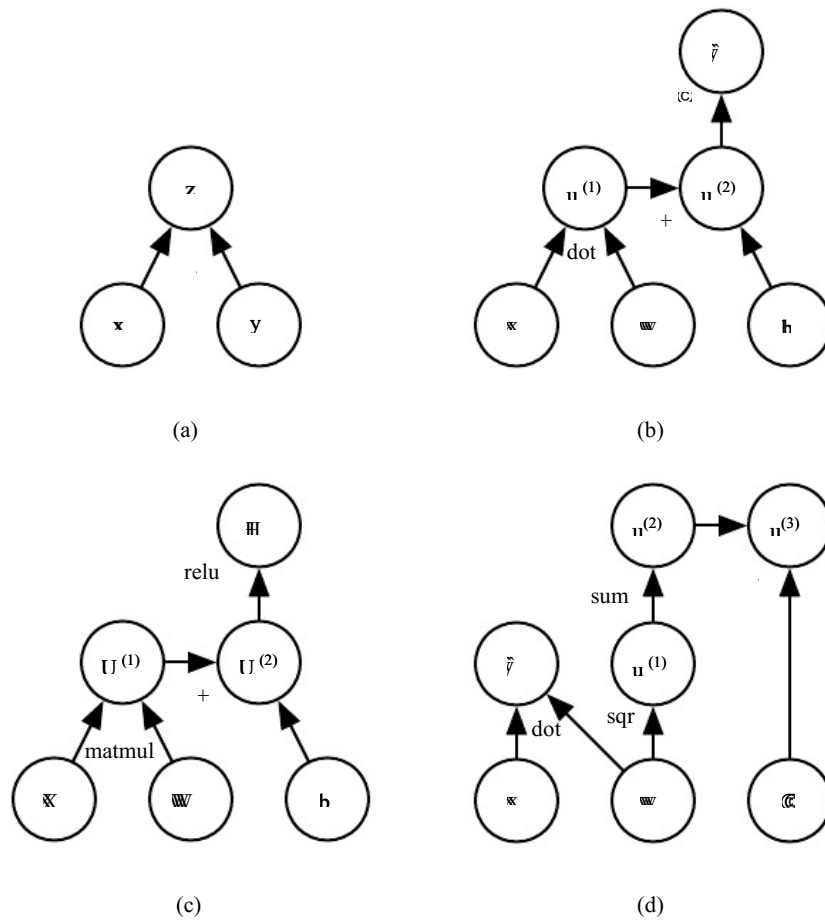
Figure 6.8: Examples of computational graphs. (a) The graph using the \times operation to compute z = xy . (b) The graph for the logistic regression prediction \hat{y} = \sigma(xw + b) . Some of the intermediate expressions do not have names in the algebraic expression but need names in the graph. We simply name the i -th such variable u^{(i)} . (c) The computational graph for the expression H = \max\{0, XW + b\} , which computes a design matrix of rectified linear unit activations H given a design matrix containing a minibatch of inputs X . (d) Examples a–c applied at most one operation to each variable, but it is possible to apply more than one operation. Here we show a computation graph that applies more than one operation to the weights w of a linear regression model. The weights are used to make the both the prediction \hat{y} and the weight decay penalty \lambda \sum_i w_i^2 .
