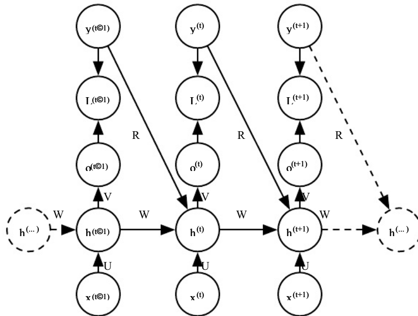
Figure 10.10: A conditional recurrent neural network mapping a variable-length sequence of x values into a distribution over sequences of y values of the same length. Compared to Fig. 10.3, this RNN contains connections from the previous output to the current state. These connections allow this RNN to model an arbitrary distribution over sequences of y given sequences of x of the same length. The RNN of Fig. 10.3 is only able to represent distributions in which the y values are conditionally independent from each other given the x values.
