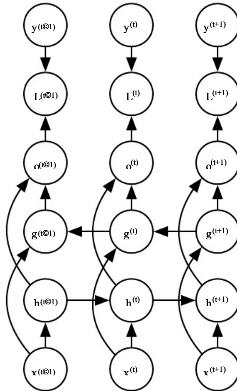
Figure 10.11: Computation of a typical bidirectional recurrent neural network, meant to learn to map input sequences x to target sequences y , with loss L^{(t)} at each step t . The h recurrence propagates information forward in time (towards the right) while the g recurrence propagates information backward in time (towards the left). Thus at each point t , the output units o^{(t)} can benefit from a relevant summary of the past in its h^{(t)} input and from a relevant summary of the future in its g^{(t)} input.
