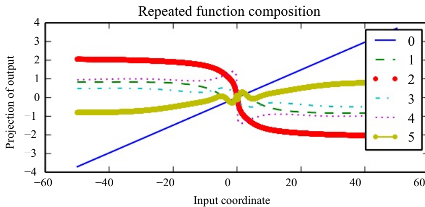
Figure 10.15: When composing many nonlinear functions (like the linear- \tanh layer shown here), the result is highly nonlinear, typically with most of the values associated with a tiny derivative, some values with a large derivative, and many alternations between increasing and decreasing. In this plot, we plot a linear projection of a 100-dimensional hidden state down to a single dimension, plotted on the y -axis. The x -axis is the coordinate of the initial state along a random direction in the 100-dimensional space. We can thus view this plot as a linear cross-section of a high-dimensional function. The plots show the function after each time step, or equivalently, after each number of times the transition function has been composed.
