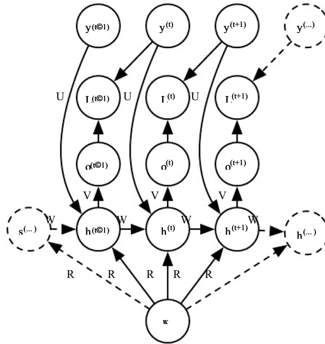
Figure 10.9: An RNN that maps a fixed-length vector x into a distribution over sequences Y . This RNN is appropriate for tasks such as image captioning, where a single image is used as input to a model that then produces a sequence of words describing the image. Each element y^{(t)} of the observed output sequence serves both as input (for the current time step) and, during training, as target (for the previous time step).
