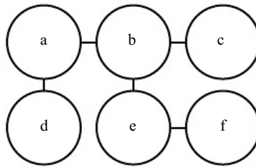
Figure 16.4: This graph implies that p(a, b, c, d, e, f) can be written as \frac{1}{Z} \varphi_{a,b}(a, b) \varphi_{b,c}(b, c) \varphi_{a,d}(a, d) \varphi_{b,e}(b, e) \varphi_{e,f}(e, f) for an appropriate choice of the \varphi functions.
