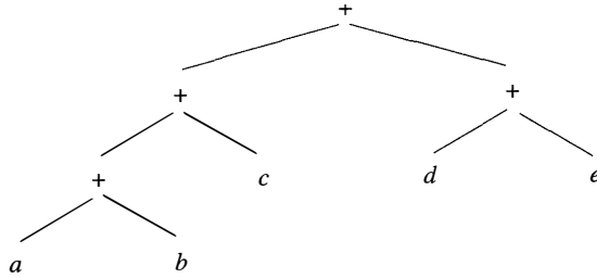
Figure 10.2: Expression tree in Example 10.3
