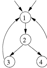
Figure 9.46: Two loops with the same header
