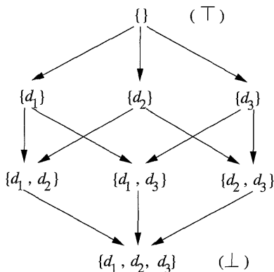
Figure 9.22: Lattice of subsets of definitions
