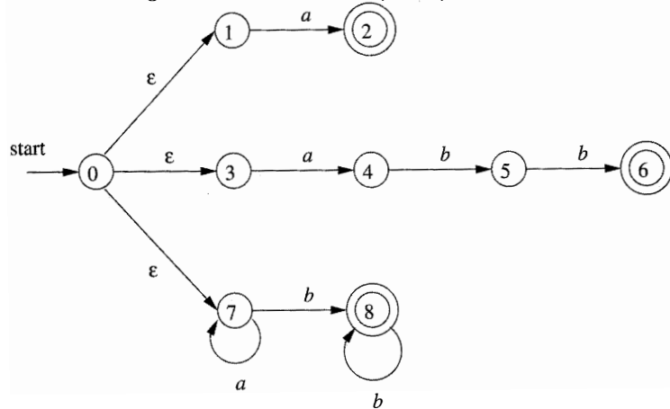
Figure 3.52: Combined NFA
