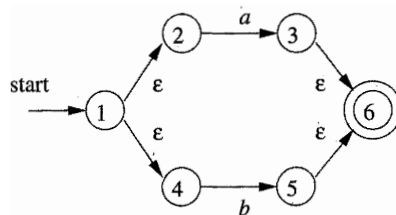
Figure 3.44: NFA for r_3
