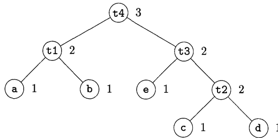
Figure 8.23: A tree labeled with Ershov numbers
