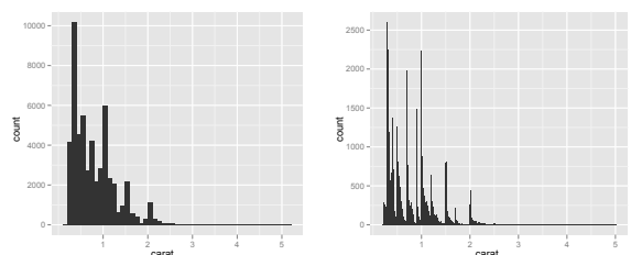
different binwidth changes the picture
