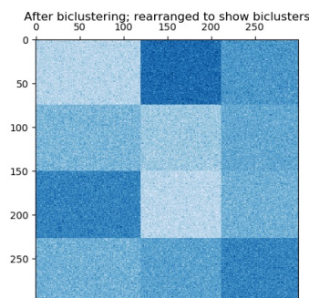
An example of checkerboard biclusters.
