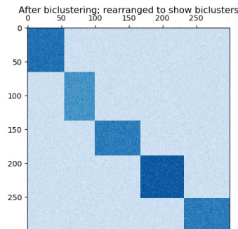
An example of biclusters formed by partitioning rows and columns.
